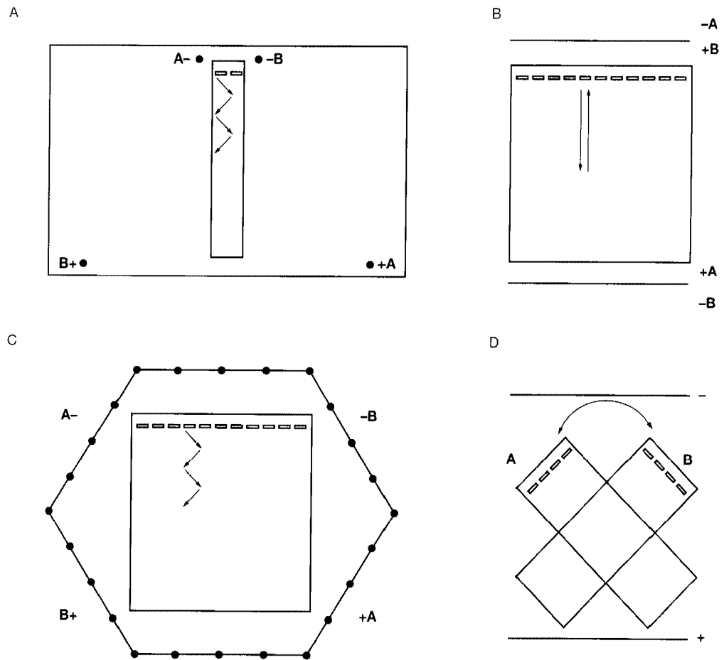
FIGURE 5-8 Pulsed-field Configurations Producing Electric Fields That Are Uniform in All Lanes of the Gel
