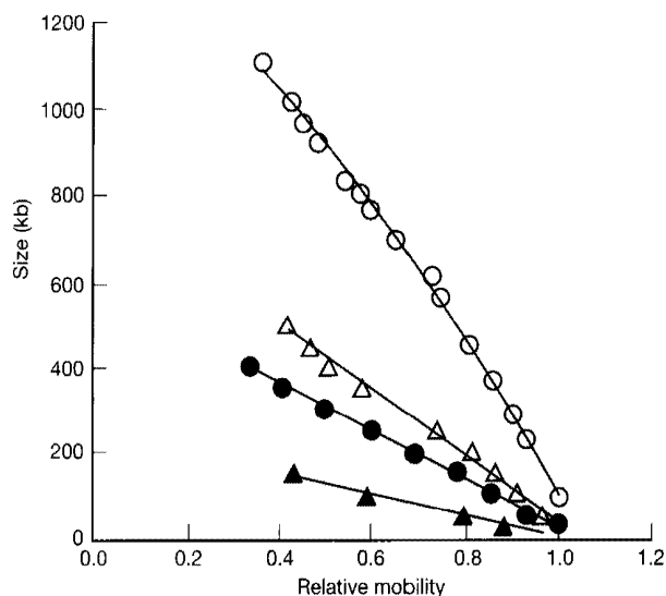
FIGURE 5-9 Effect of Pulse Time on Migration of DNA through a Pulsed-field Gel
