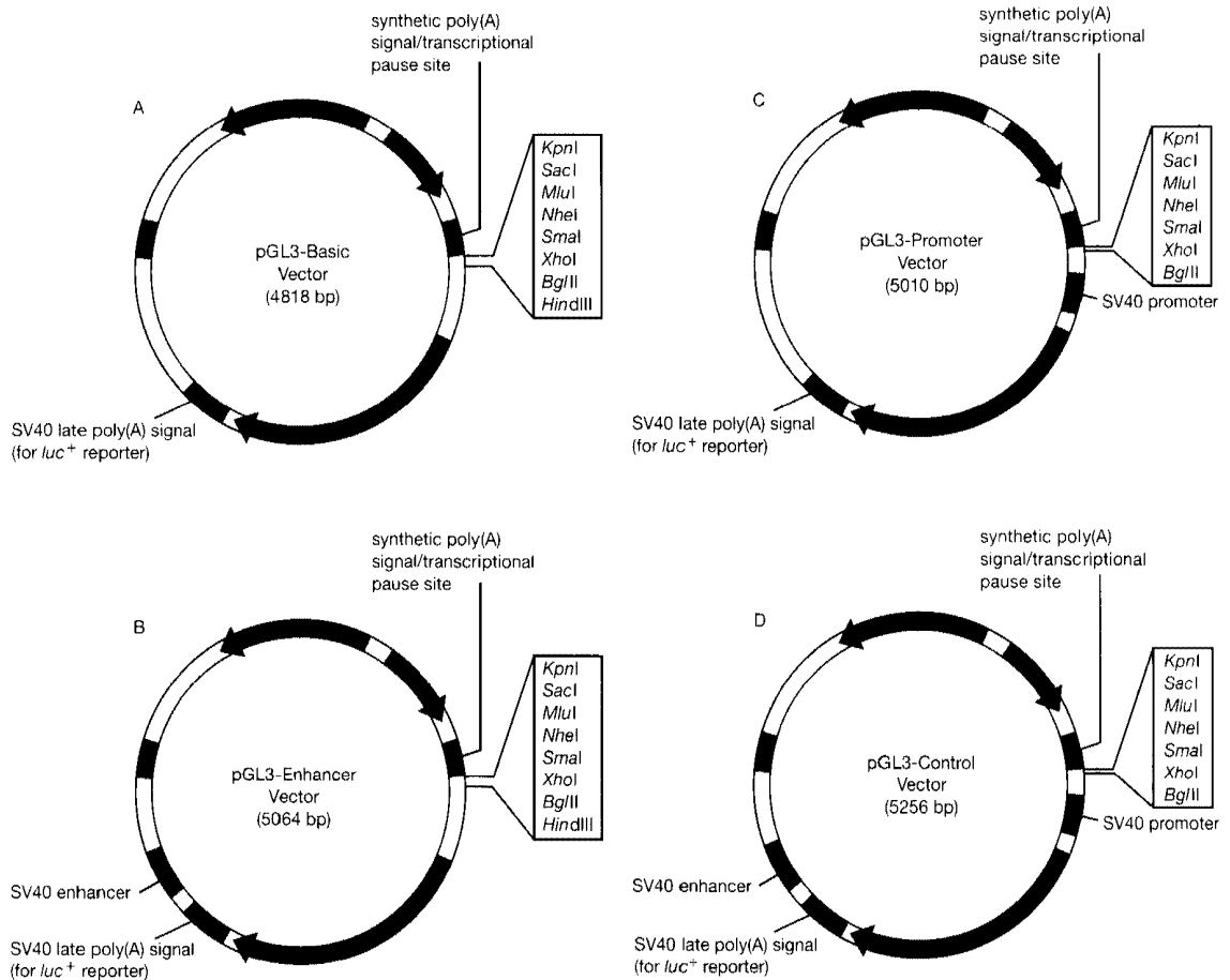
FIGURE 17-4 pGL3 vectors
