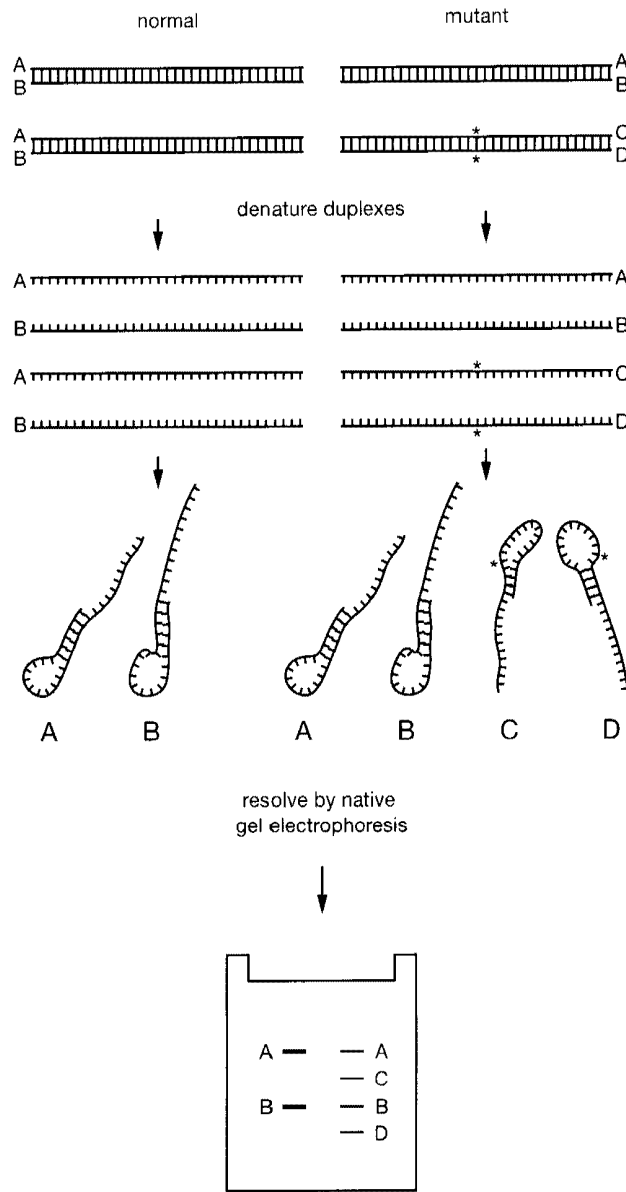
FIGURE 13-6 Schematic for Single-stranded Conformational Polymorphism
