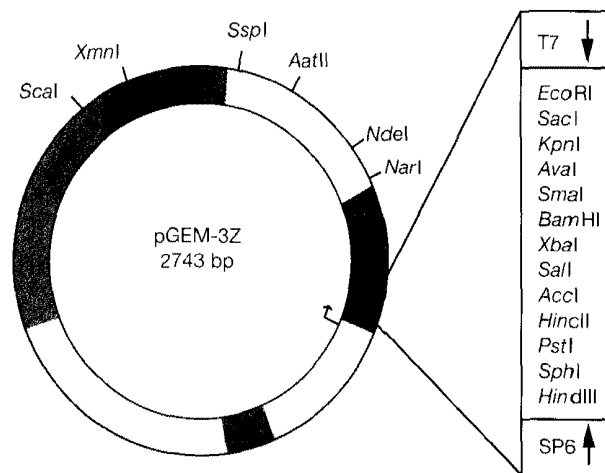
FIGURE 15-4 pGEM-3Z Vector
