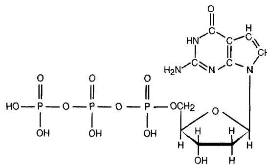
FIGURE 12-13 Structure of the Nucleotide Analog 7-deaza-dGTP
