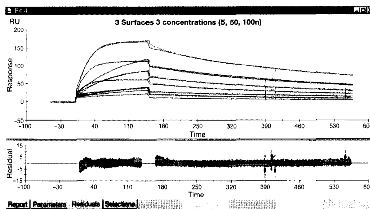
FIGURE 18-30 Global Fitting of the Binding Model
