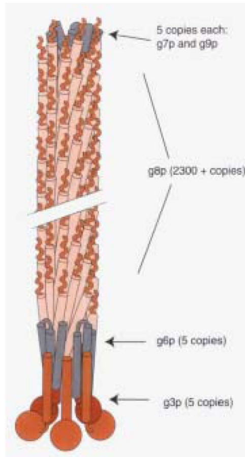
FIGURE 3-3 Structural Model of an M13 Particle
