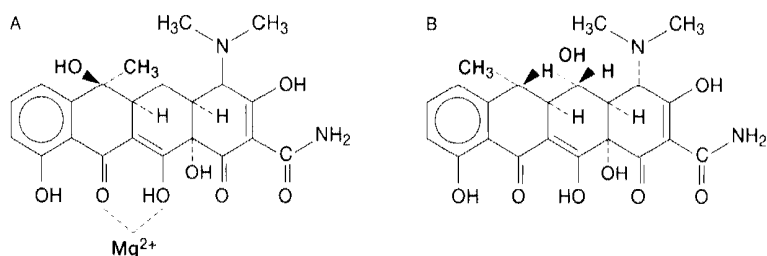
FIGURE 17-6 Structure of Tetracycline and Doxycycline
