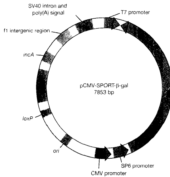
FIGURE 16-2 pCMV-SPORT-β-gal
