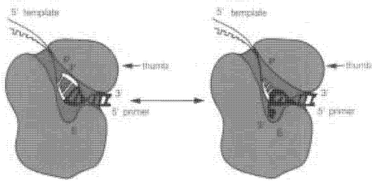
FIGURE 9-6 A Model of DNA Bound to the Klenow DNA Polymerase
