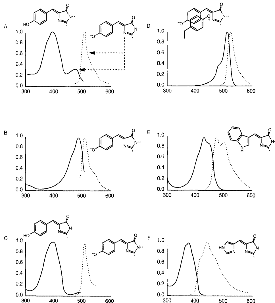
FIGURE 17-12 Fluorescence Excitation and Emission Spectra for GFP Variants
