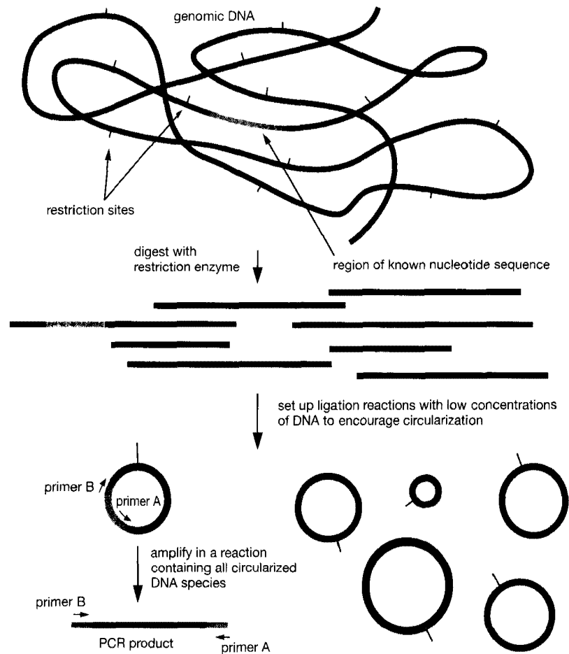
FIGURE 8-7 Schematic Representation of Inverse PCR
