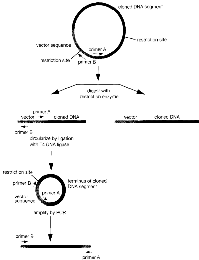
FIGURE 4-14 Inverse PCR
