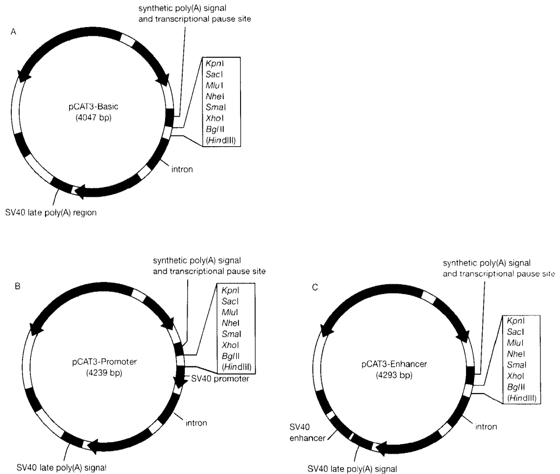
FIGURE 17-3 pCAT3 Vectors
