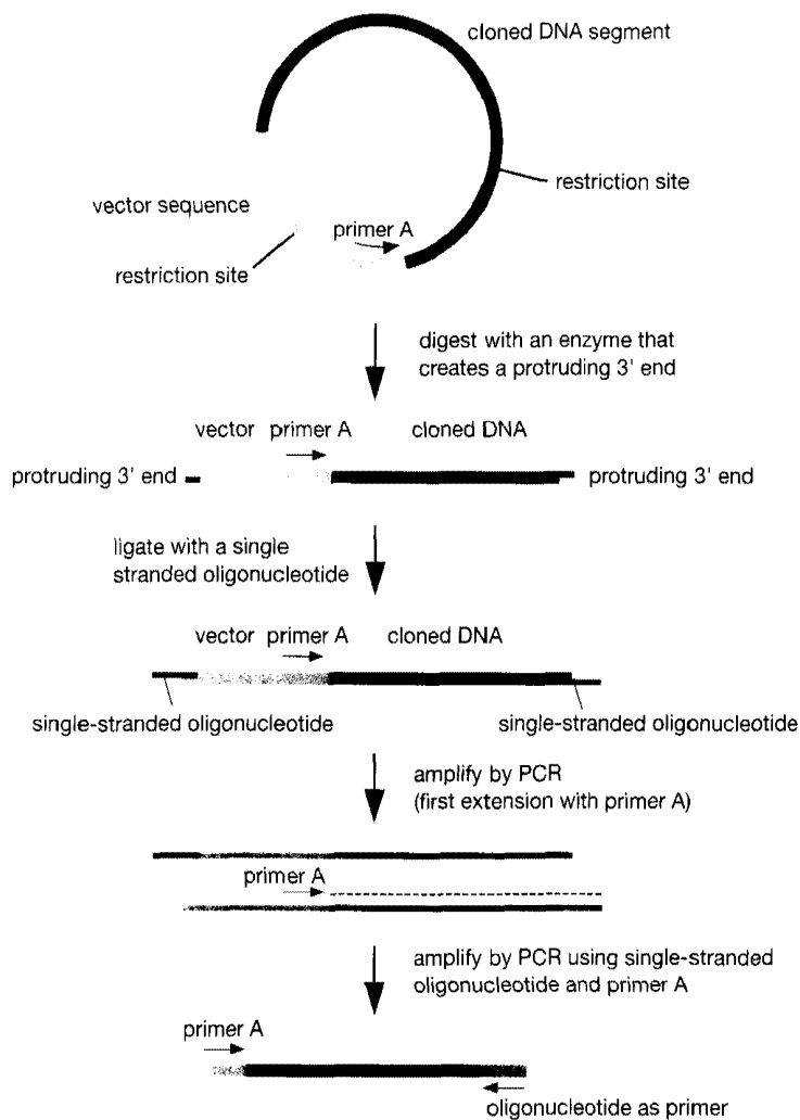
FIGURE 4-16 Single-site Scheme
