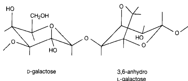
FIGURE 5.1 Chemical Structure of Agarose
