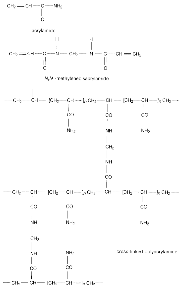
FIGURE 5-6 Structure of Polyacrylamide
